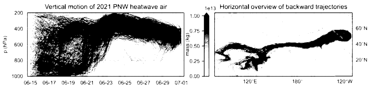
Times series plots depicting the initial upward and later downward motion of the air that would later become entrained by the persistent and extreme high pressure system that precipitated the historic 2021 heat event as it moved from the subtropical western Pacific Ocean to the Pacific Northwest interior. Adapted from Schumacher et al. 2022.
