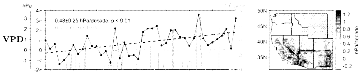
Left: Time series plot depicting observed increases in the vapor pressure deficit (VPD) over the Western United States. Right: Map plot depicting observed historical increases in VPD over the same period used in the time series plot at left. Adapted from Zhuang et al. 2021.
