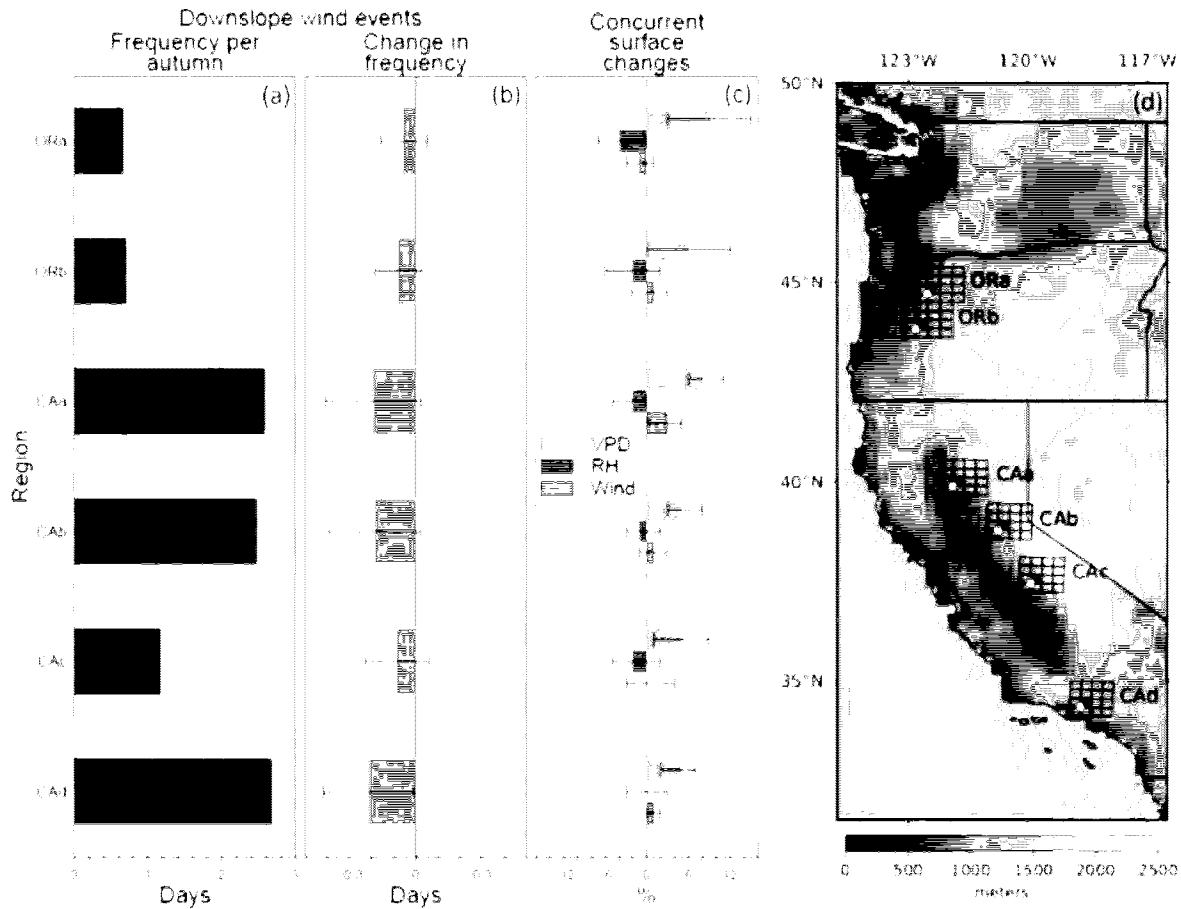
Panels a) and b) depict projected historical changes in the frequency of autumn “offshore wind” events along different portions of the West Coast of the United States. Panel c) depicts projected historical changes in the intensity of offshore wind events in addition to trends in autumn relative humidity (RH) and vapor pressure deficit (VPD). Apparent are small decreases in the magnitude and frequency of offshore winds but substantial increases in the VPD in western Oregon. Adapted from Hawkins et al. 2022.
