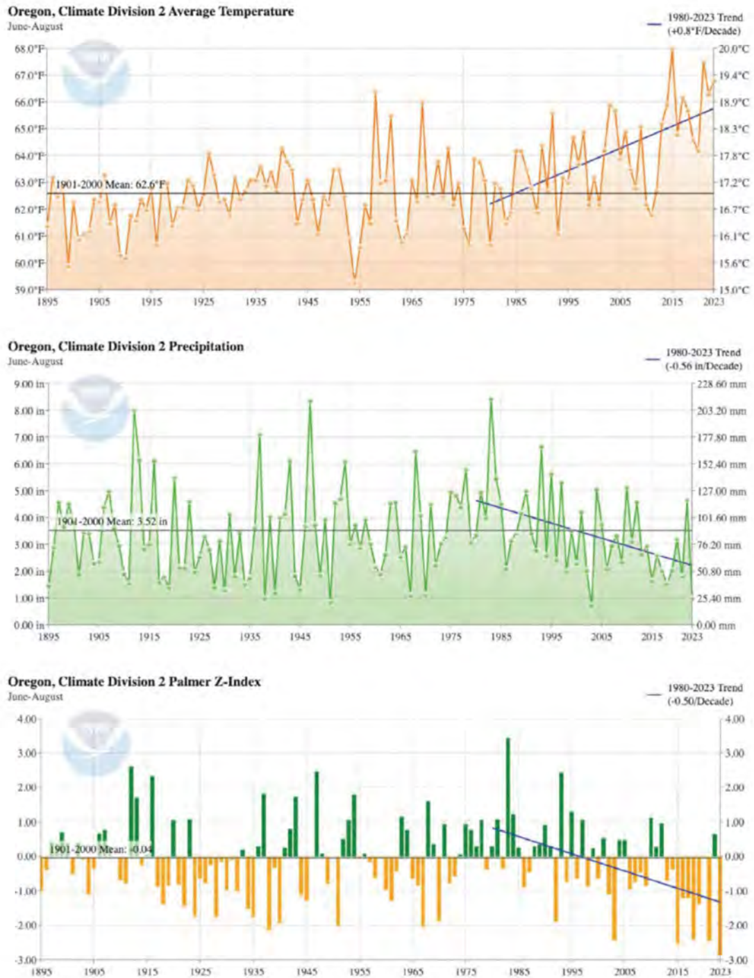
Time series plots depicting historically observed summer (Jun-Aug) temperatures (top), summer precipitation (middle), and summer drought severity (as measured by the normalized Palmer Index; bottom). In each plot, linear trends for the period 1980-2023 are shown. Data via NOAA's "Climate at a Glance" portal.
